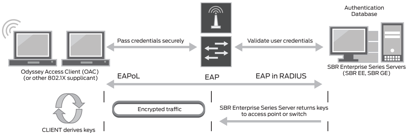
Figure 1: SBR Enterprise Series Steel-Belted Radius Servers in an 802.1X network environment
