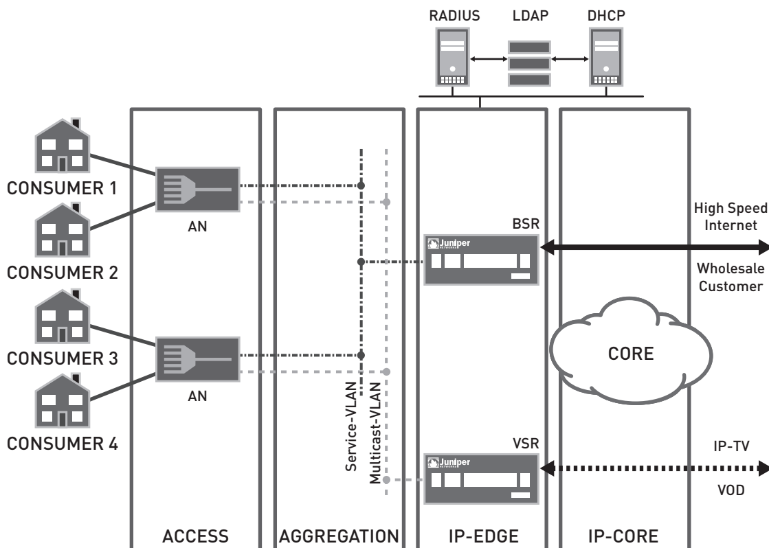
Figure 2: S-VLAN design for multi-edge networks
