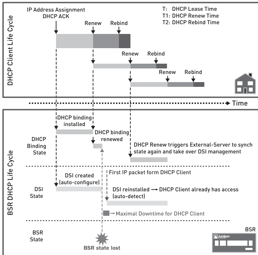
Figure 6: Implications of loss of DHCP state
