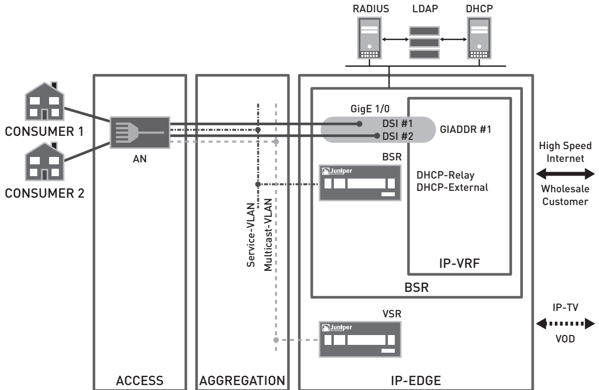
Figure 3: Dynamic subscriber interface
