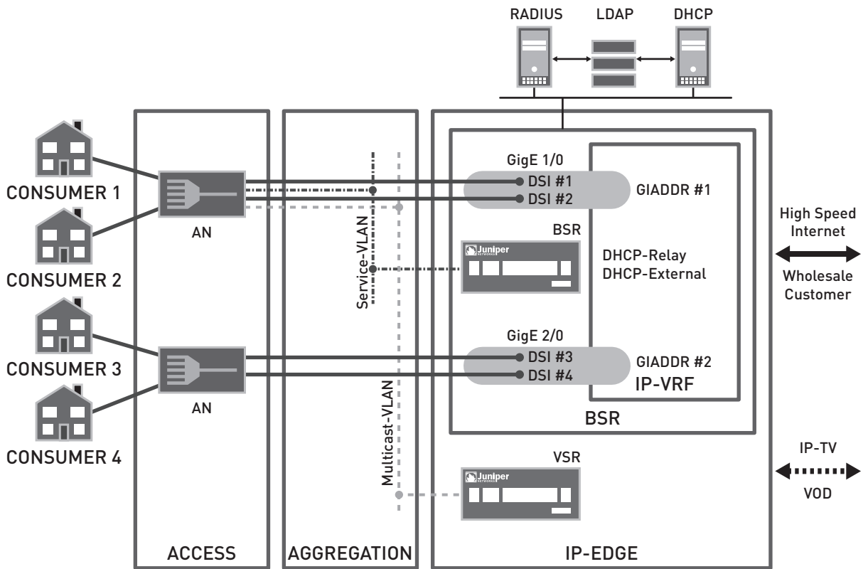
Figure 5: Architecture for scaling the S-VLAN model
