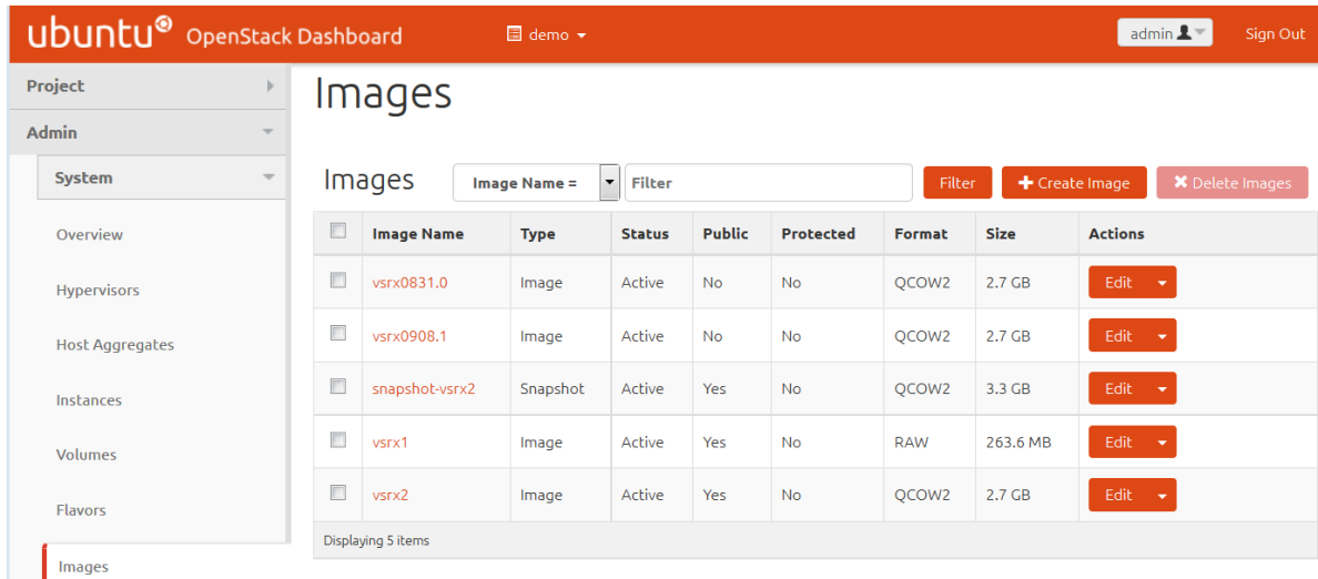
Figure 60: OpenStack Images
