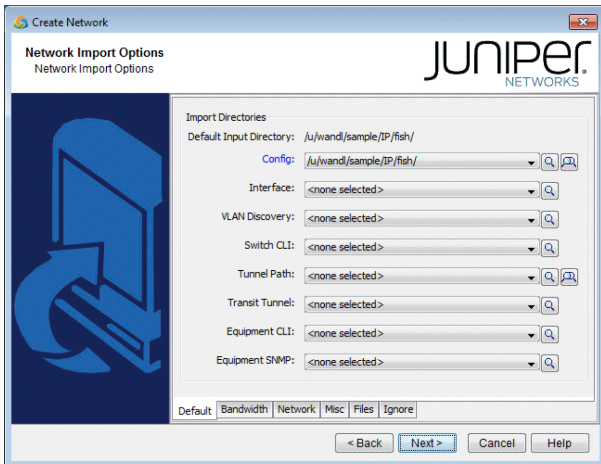
Figure 4: Selecting the Output Directory and Runcode
