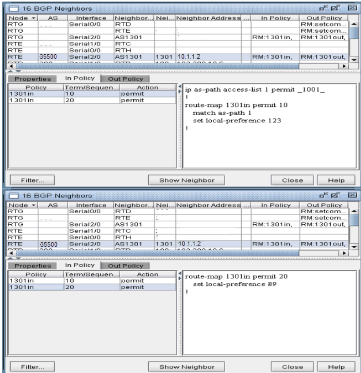
Figure 71: BGP In Policy for RTE
