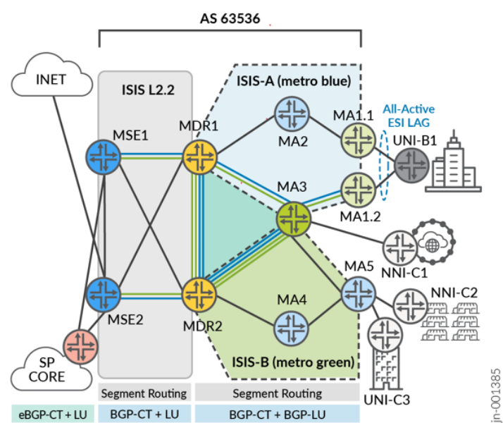
Figure 3: Metro Multi-Ring Topology
