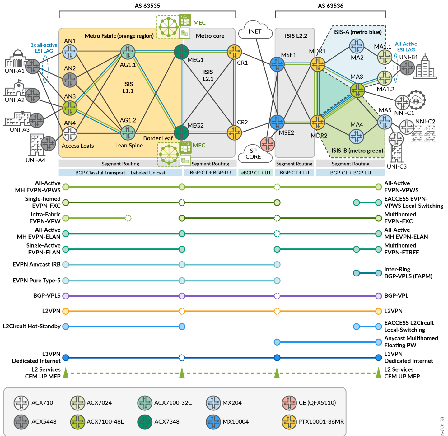
Figure 44: Metro Fabric to Multi-Ring Inter-AS Topology
