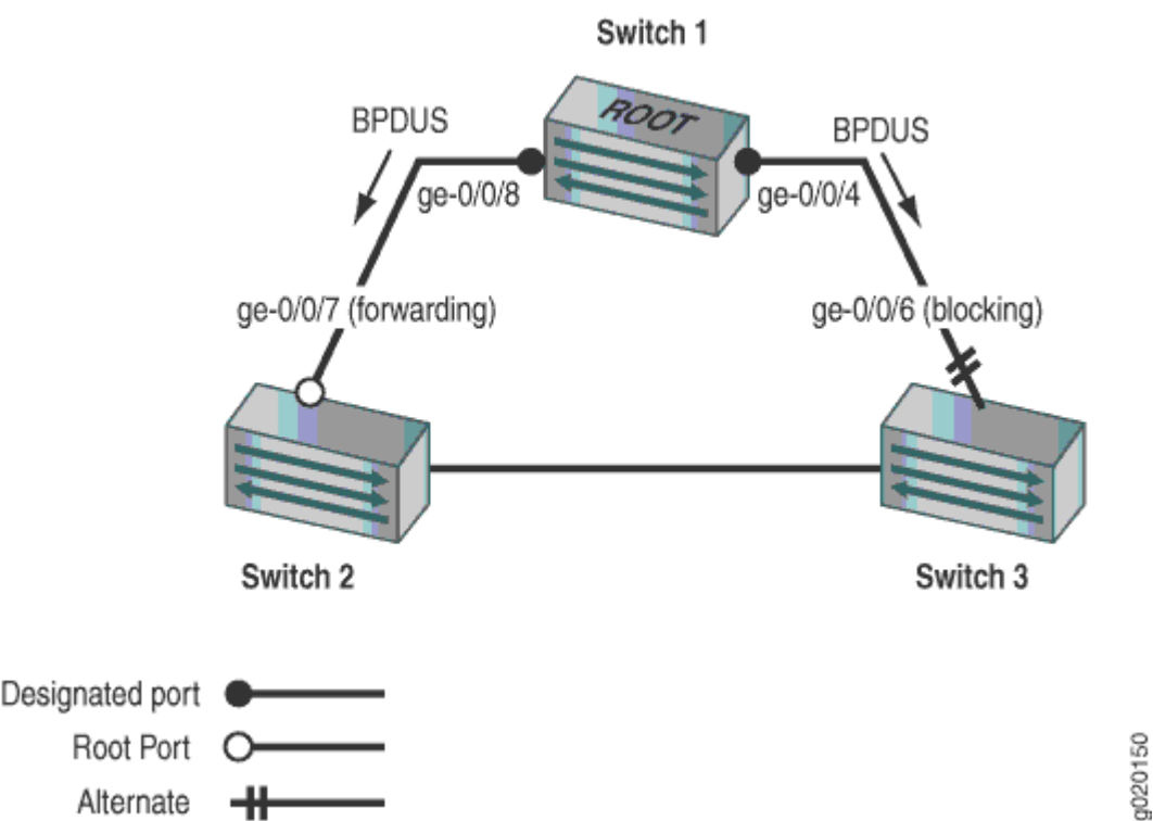
Figure 11: Network Topology for Loop Protection
