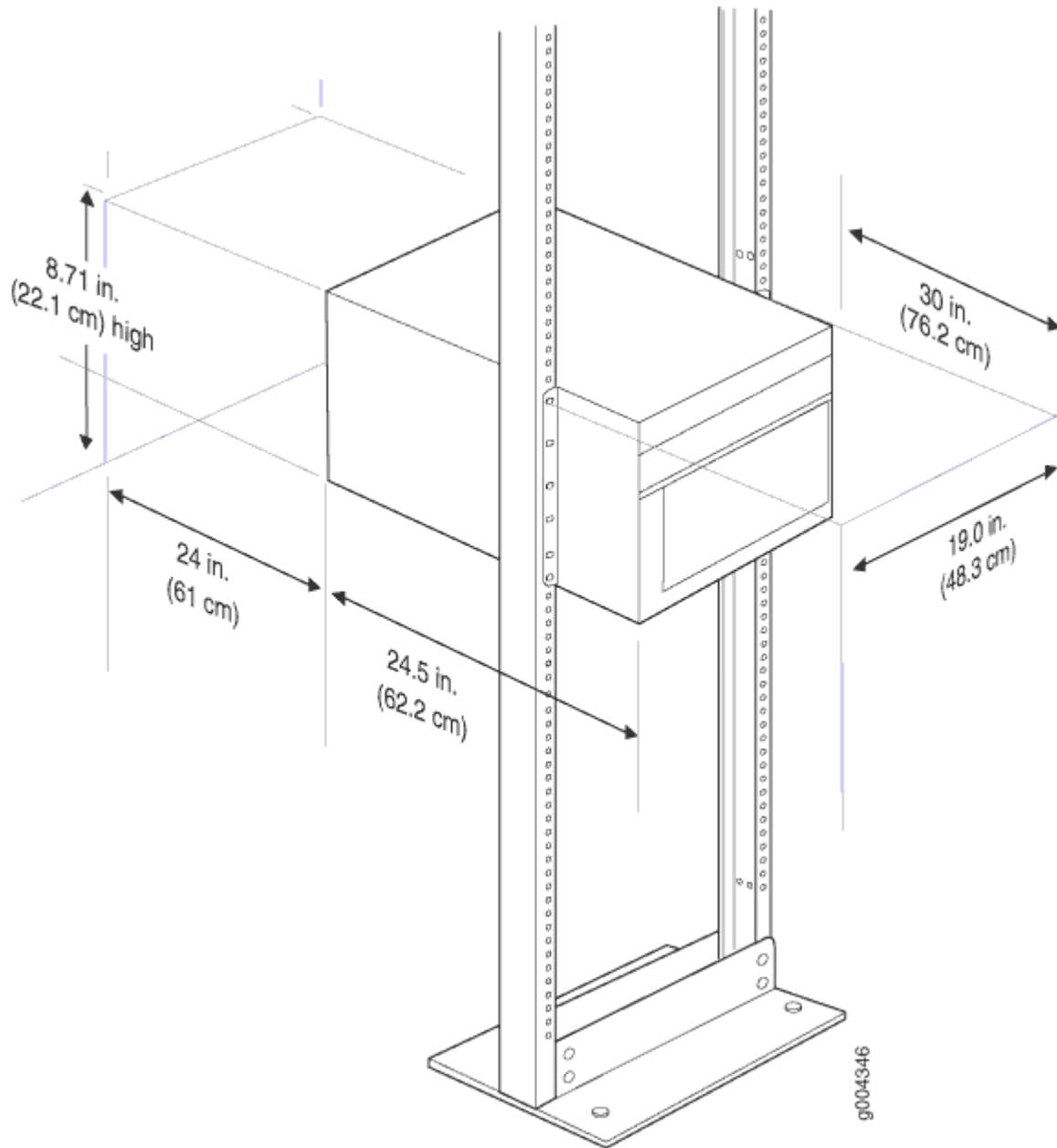
Figure 1: MX240 Rack Clearance and Router Dimensions
