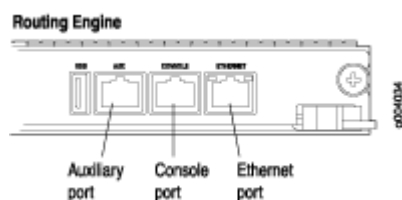
Figure 8: Routing Engine Management Ports
