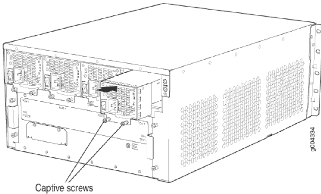
Figure 10: Installing an AC Power Supply
