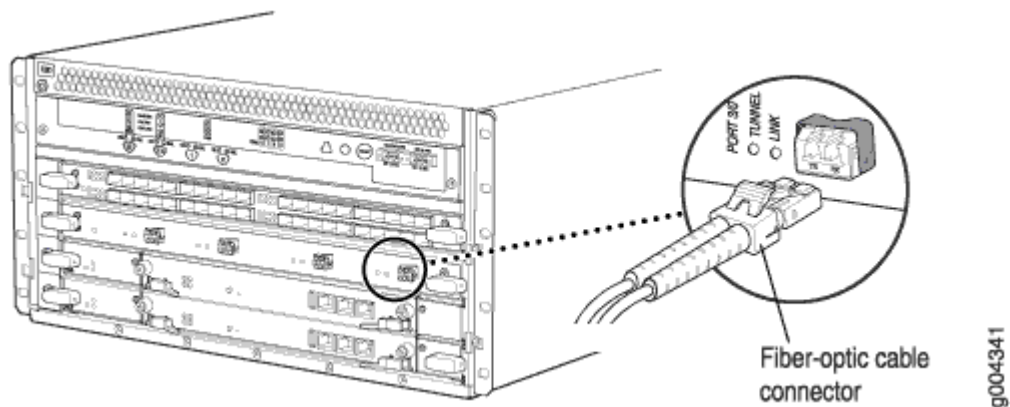
Figure 9: Connect DPC Cables
