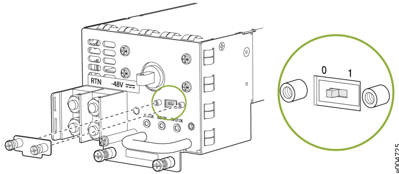
Figure 12: DC High-Capacity Power Supply Input Mode Switch
