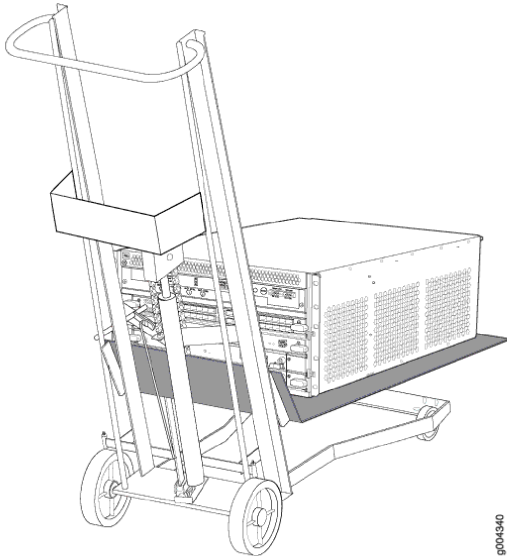
Figure 6: Load the MX240 Router onto the Lift
