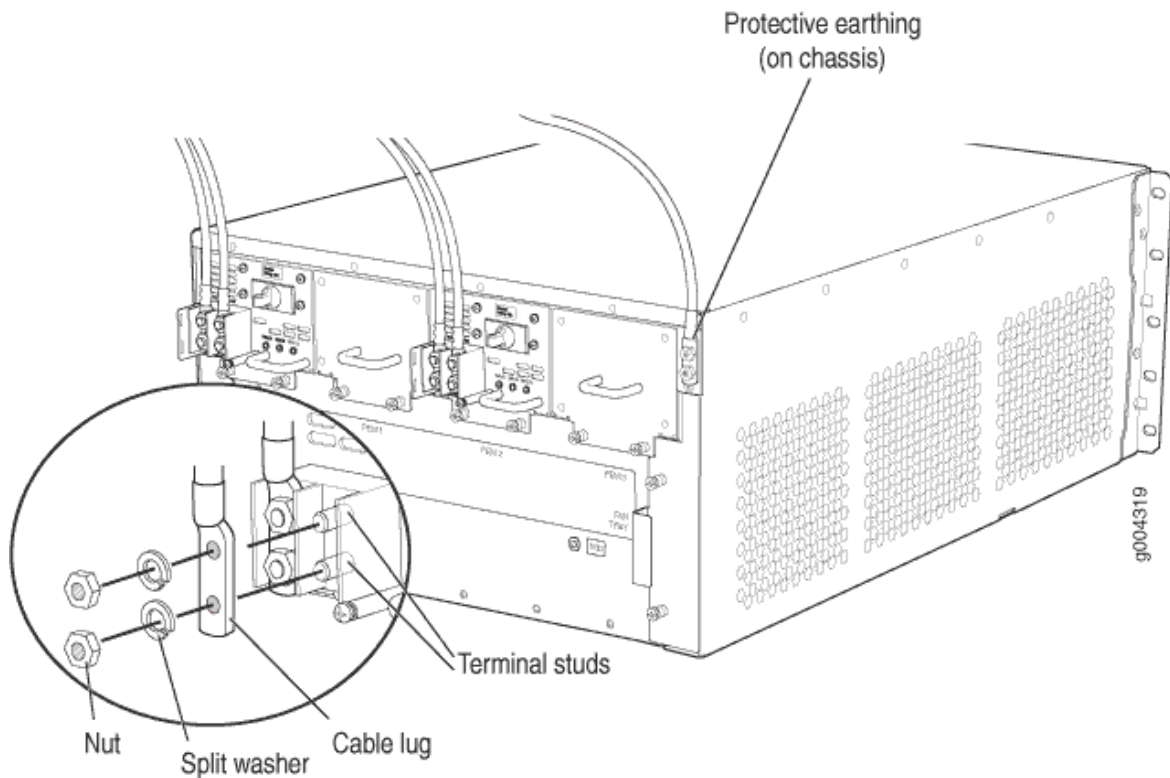
Figure 11: Connect Power Cables
