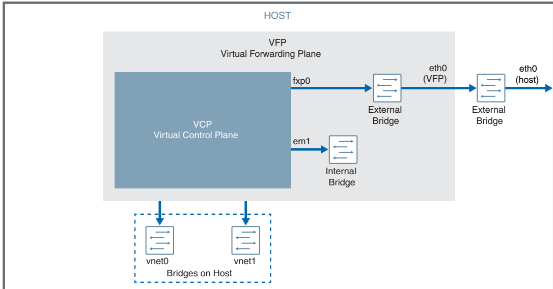
Figure 4: Nested VM with virtio Interfaces
