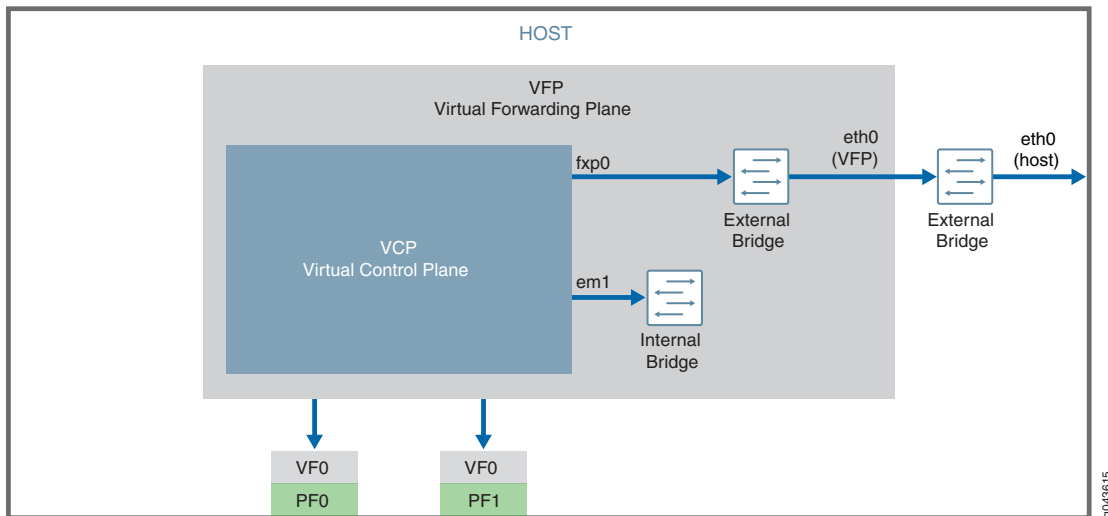
Figure 5: Nested VM with SR-IOV Interfaces
