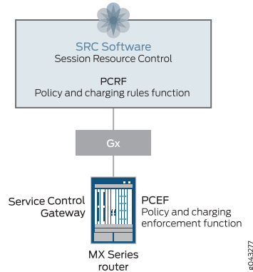
Figure 1: Interface Between the SRC software and the Services Control Gateway
