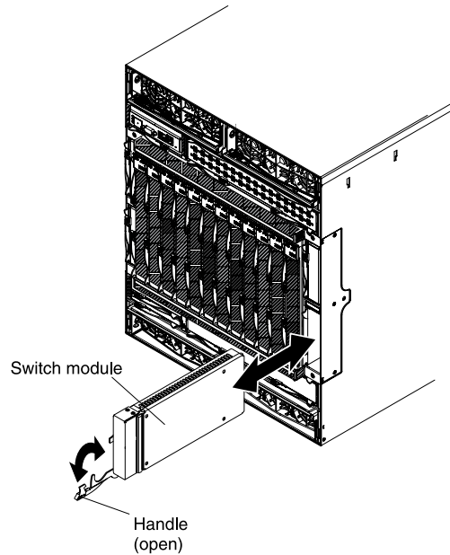
Figure 1: Removing and Installing a JCS 1200 Switch Module
