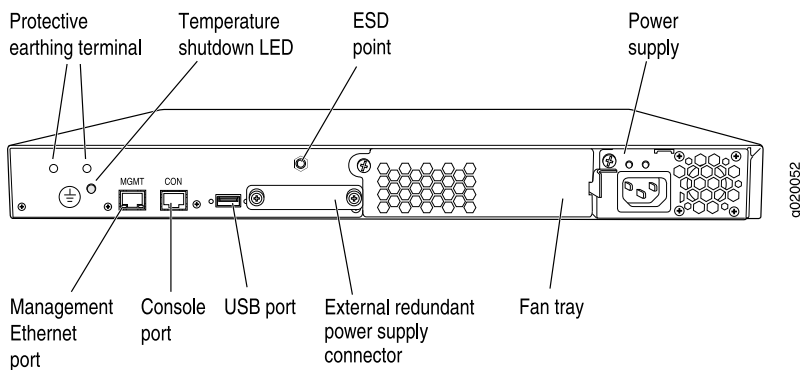
Figure 1: EX 3200 Switch Rear Panel
