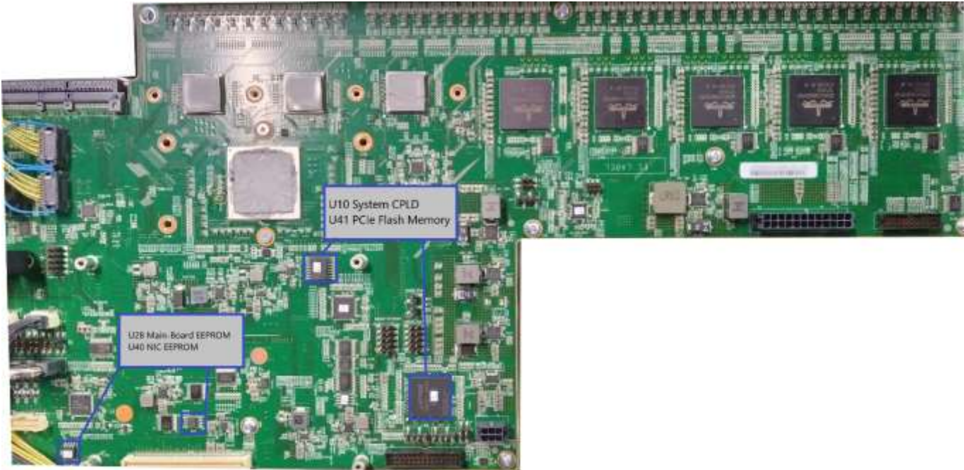
Figure 3-7: Locate System-CPLD, PCIe flash NIC IDEEPROM and MB-IDEEPROM.
