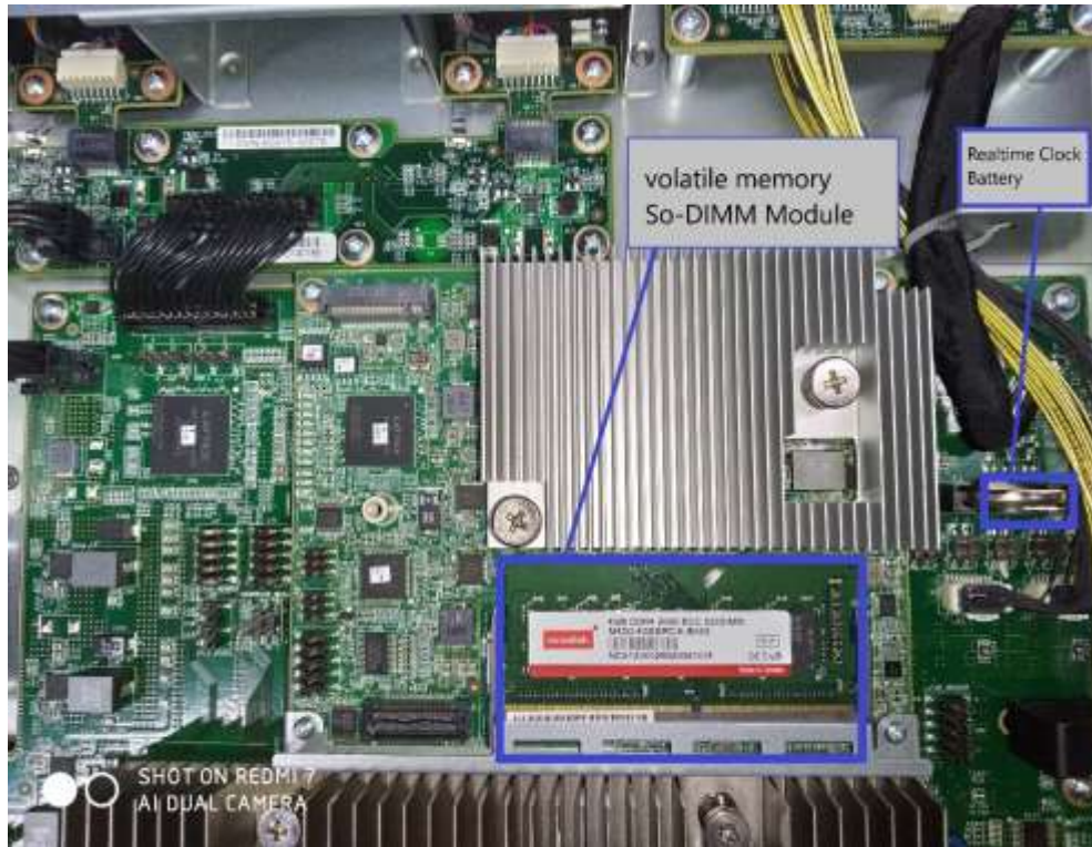
Figure 3-4: Locate DIMM and Battery
