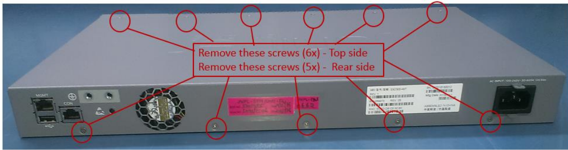
Figure 3-1: Top and rear side screws
