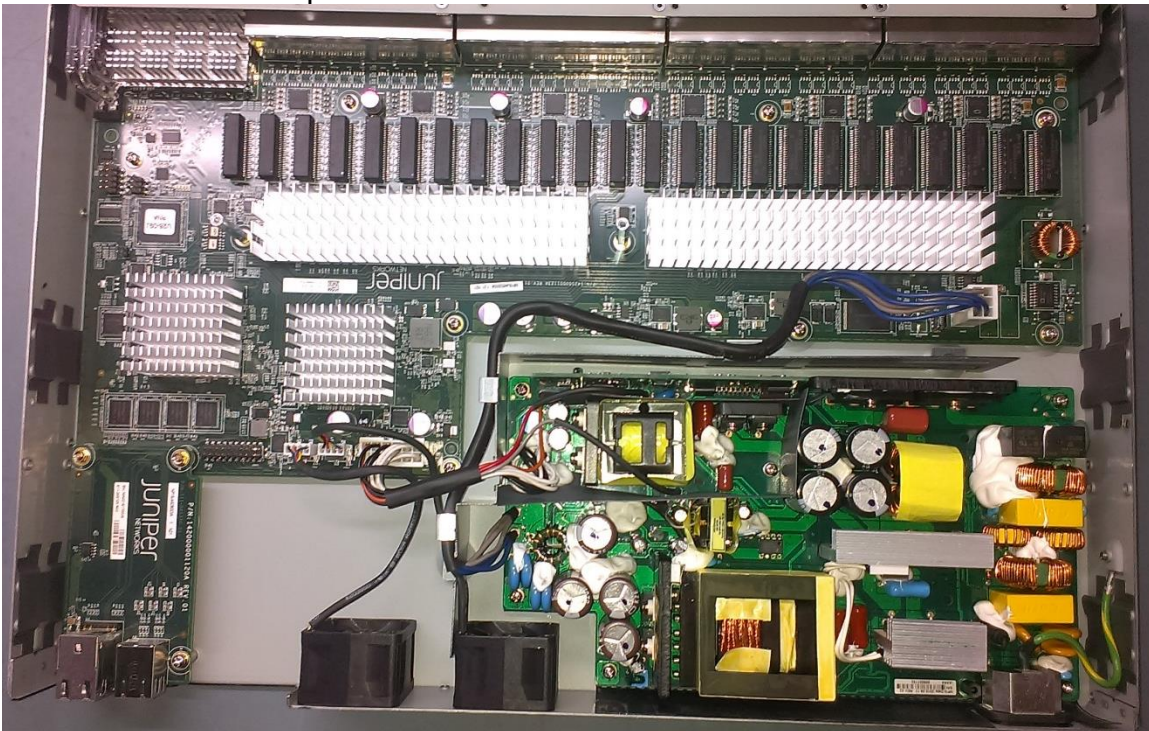
Figure 3-4: Open Chassis, Sazerac-48P
