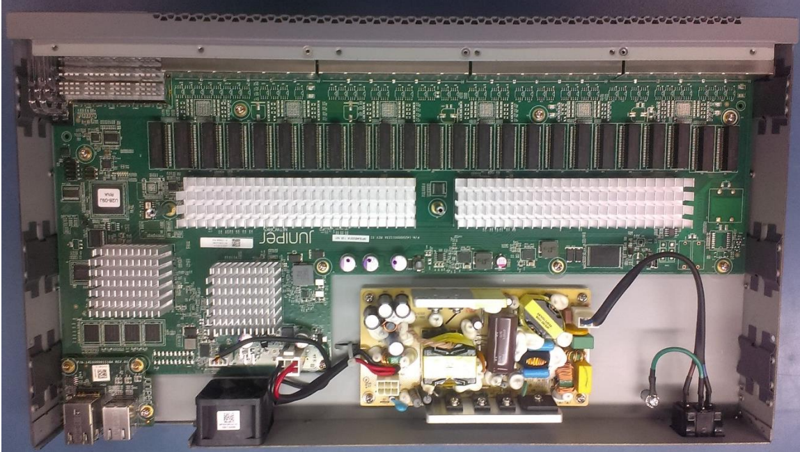
Figure 3-5: Open Chassis, Sazerac-48T
