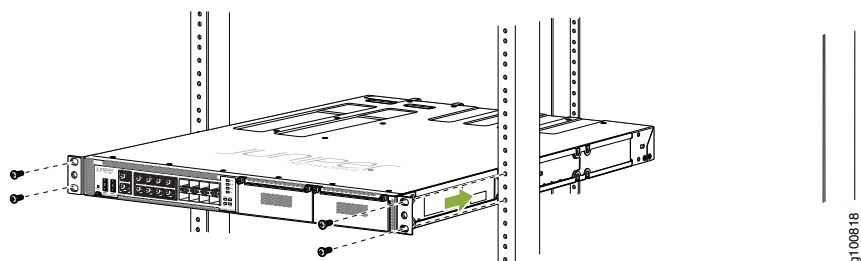
Figure 3: Attaching the Device to the Rack
