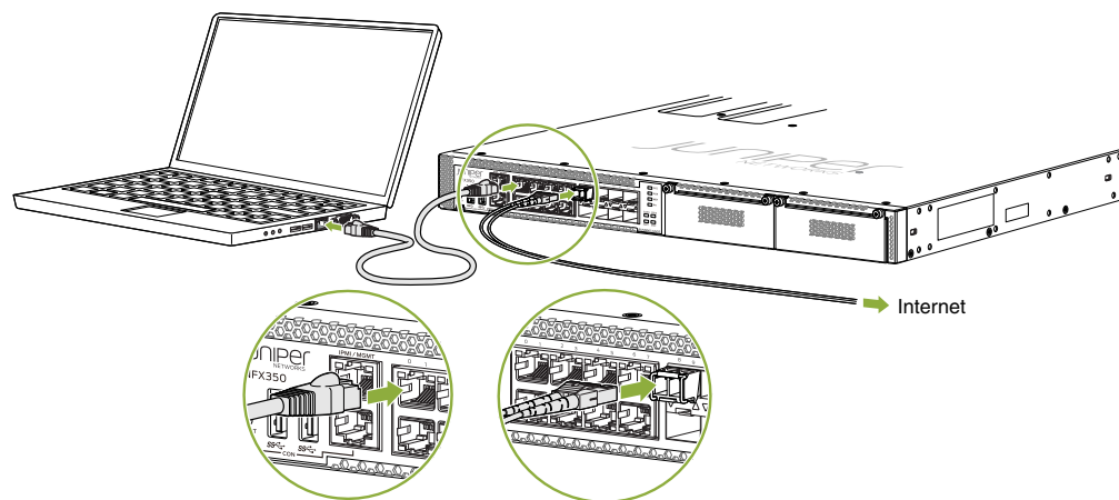
Figure 4: Connecting the Interfaces on an NFX350 Device
