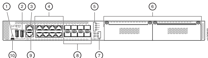
Figure 1: Front Panel Components of NFX350
