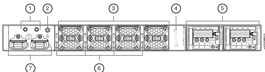
Figure 2: Rear Panel Components of NFX350
