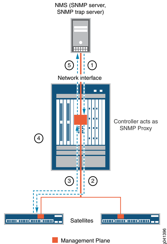
Figure 6: SNMP Get Process
