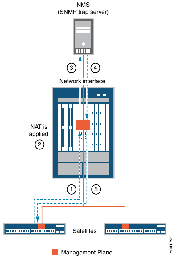
Figure 7: SNMP Trap Process
