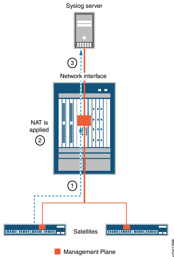
Figure 8: System Logging Collection Process
