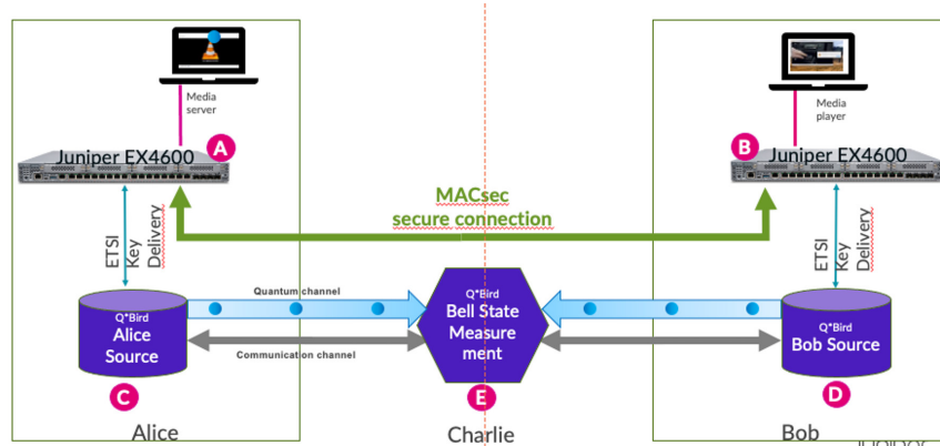
Figure 3.1 MDI-QKD
