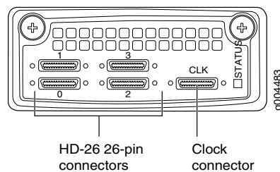
Figure 1: CTP150 Serial Multiservice Interface Module
