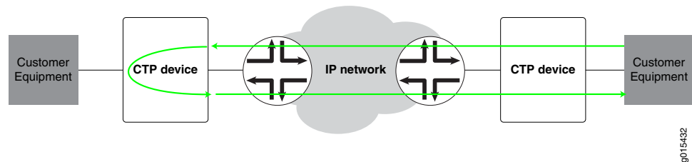
Figure 3: Serial Loop to the Network
