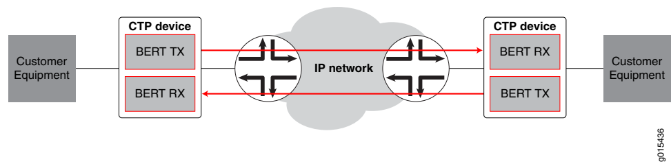
Figure 7: End-to-End BERT Transmission and Reception
