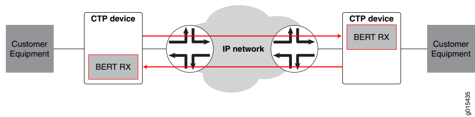
Figure 6: End-to-End BERT Reception
