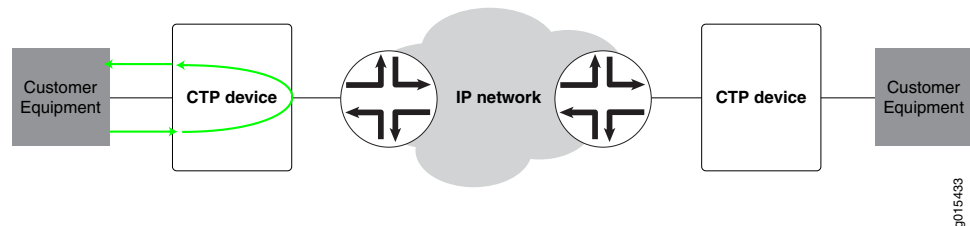
Figure 2: Serial Loop to the Interface
