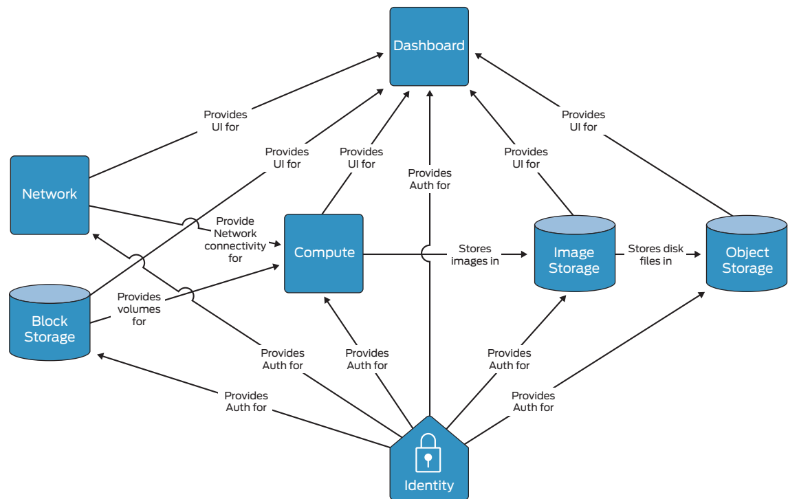
Figure 1: OpenStack components. Source: openstack.org
