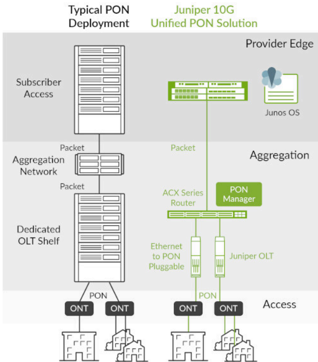
Figure 3: Legacy versus Juniper Unified PON solution
