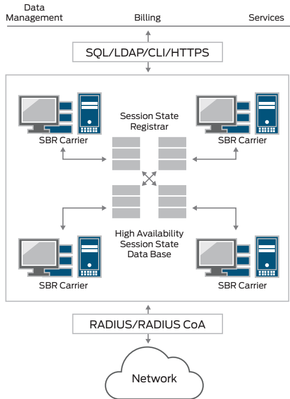
Figure 2: SBR Carrier with its SSR module deployed in a cluster configuration
