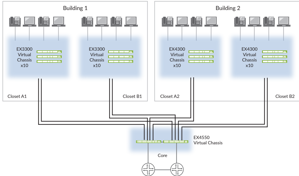
Figure 4: Small to medium-sized enterprises with Virtual Chassis technology
