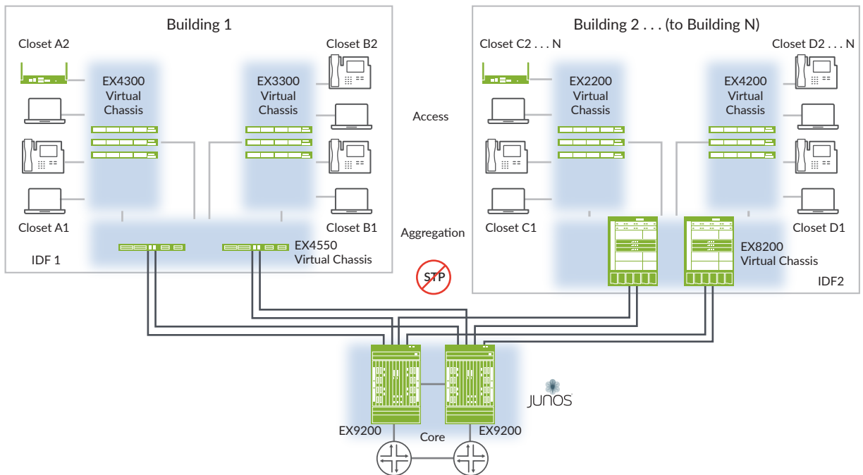
Figure 5: Large enterprise network with Virtual Chassis technology
