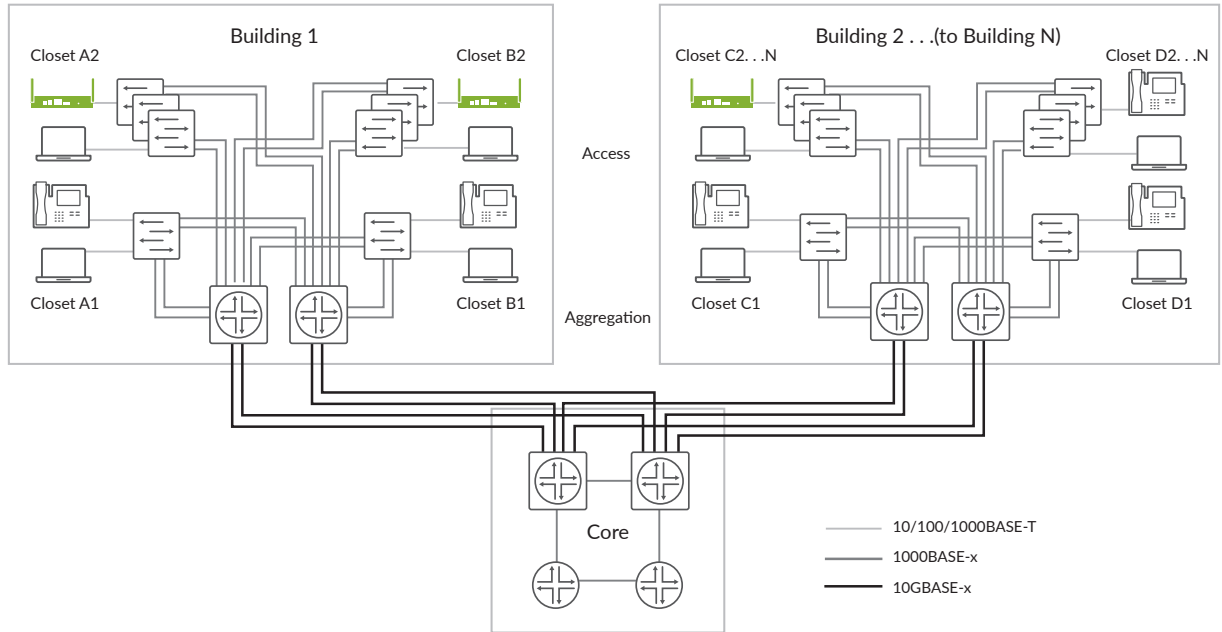
Figure 2: Traditional enterprise network
