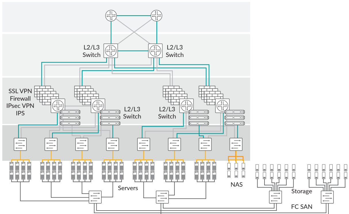
Figure 1: Legacy data center architecture
