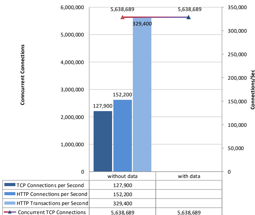
Figure 10 – Maximum Capacity (Concurrency and Connection Rates)
