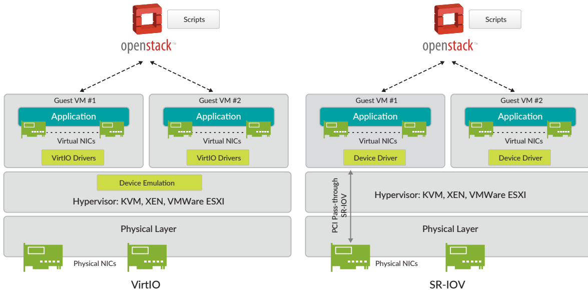
Figure 1: The vMX architecture for VirtIO and SR-IOV.
