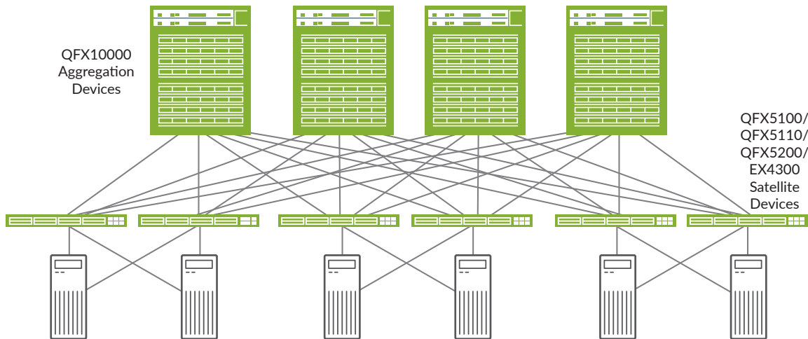
Figure 1: Junos Fusion Data Center deployment.
