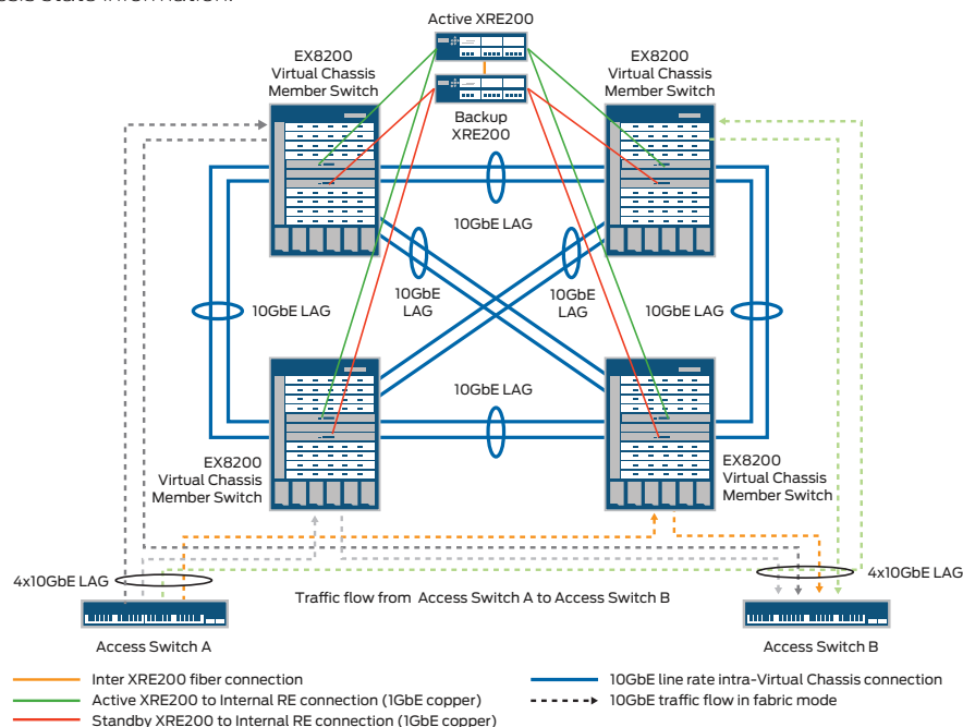
Figure 1: Example of a four-member EX8200 Virtual Chassis configuration
