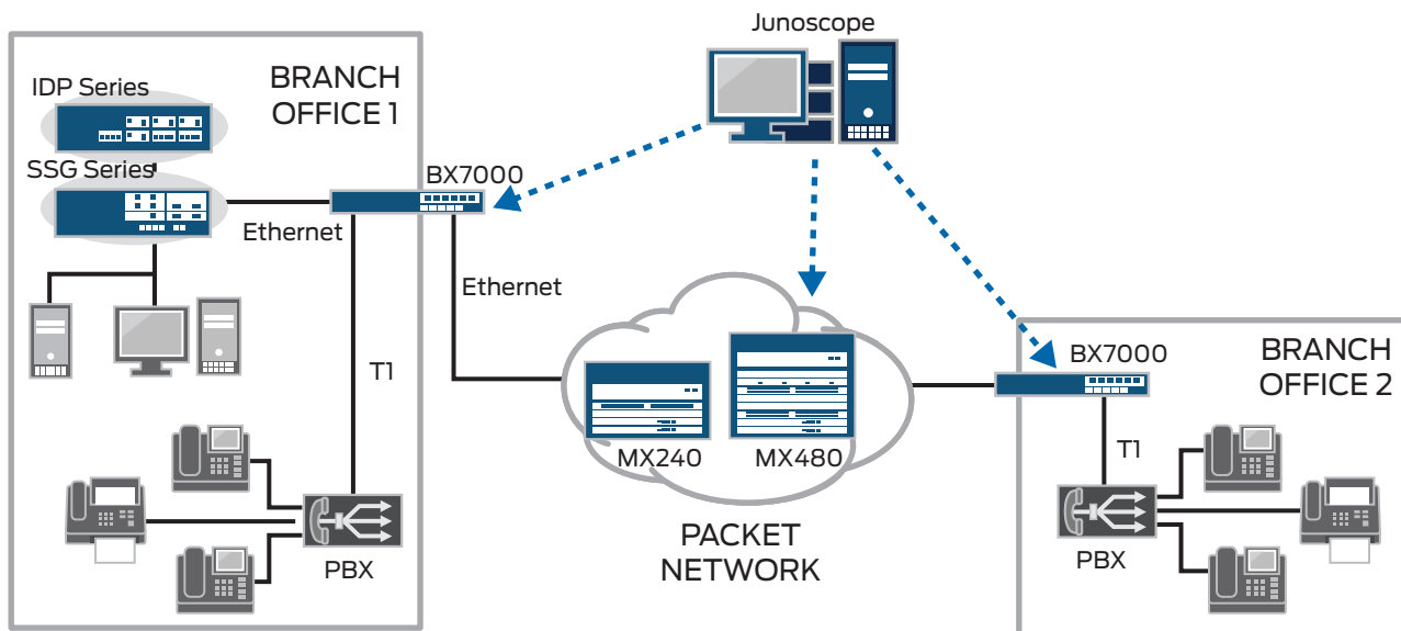
Figure 3: PBX interconnect between branch offices
