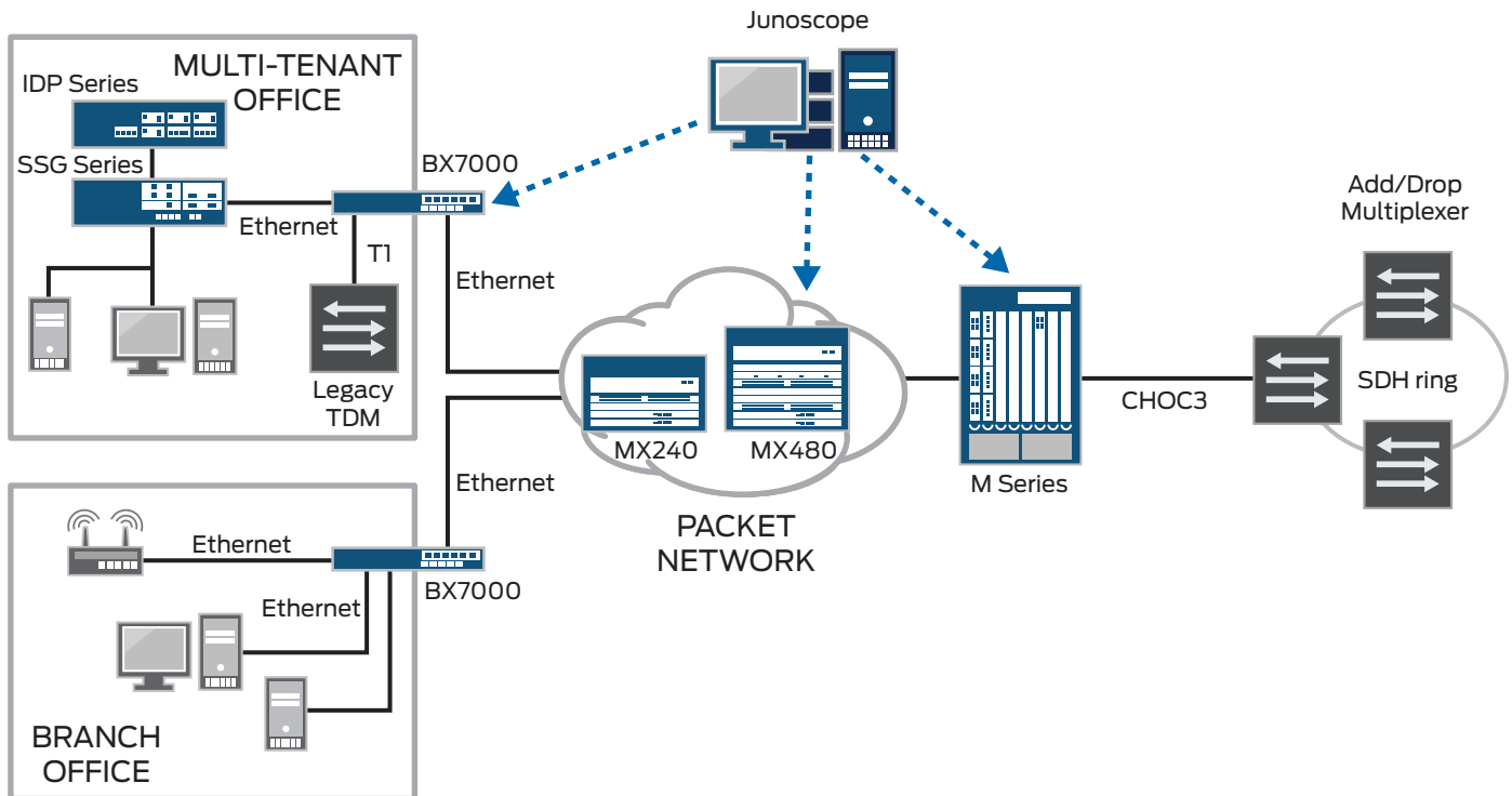
Figure 1: Legacy leased line service over IP/MPLS
