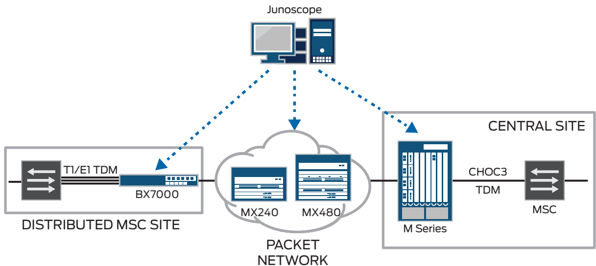
Figure 2: Mobile Switching Center (MSC) site interconnect
