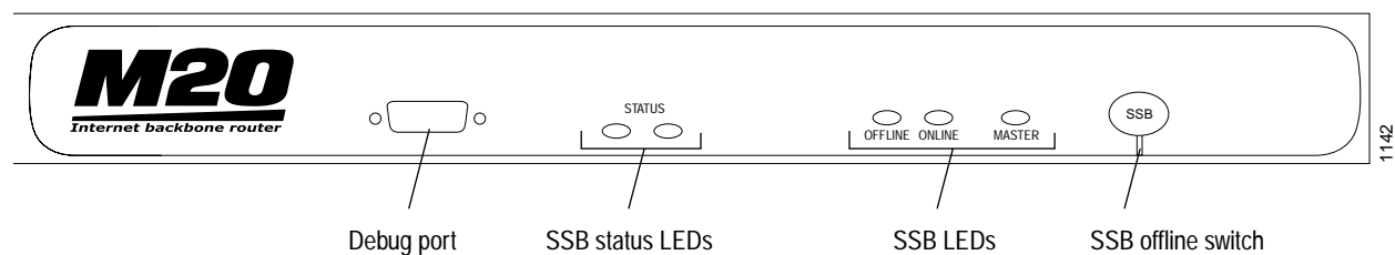
Figure 166: SSB LEDs
