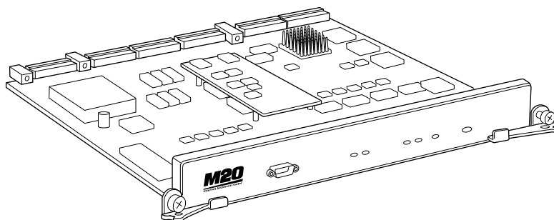
Figure 164: SSB Component
