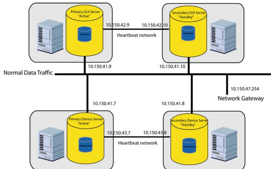
Figure 3: Extended HA Configuration Example
