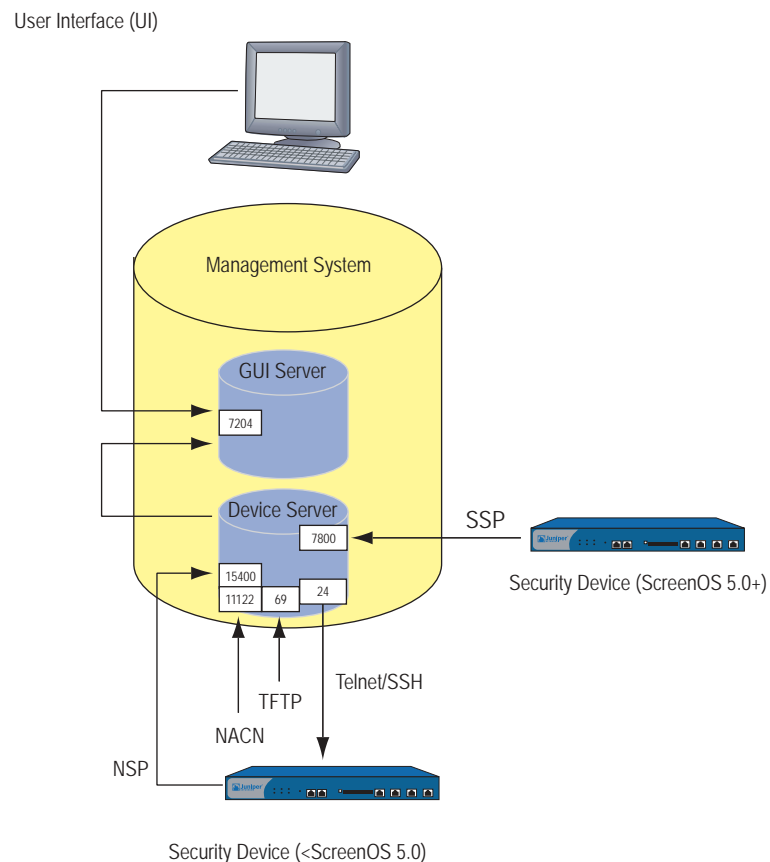
Figure 6: NetScreen-Security Manager Communications
