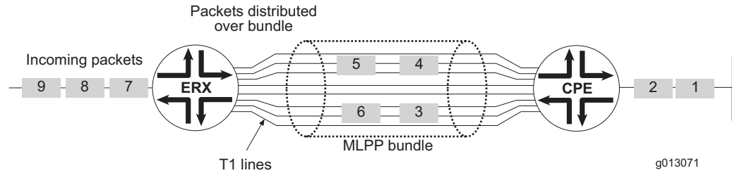
Figure 20: MLPPP Aggregation of T1 Lines into a Single Bundle
