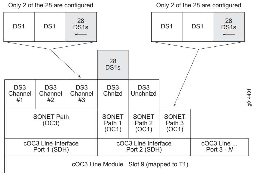
Figure 15: cOC3 Line Module Stacking Example
