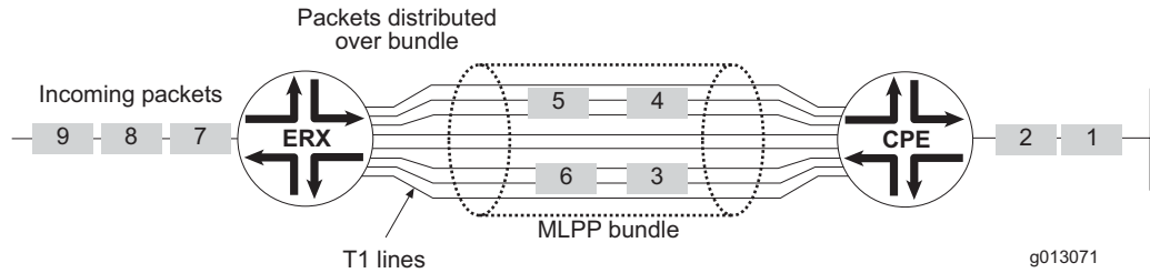
Figure 17: MLPPP Aggregation of T1 Lines into a Single Bundle
