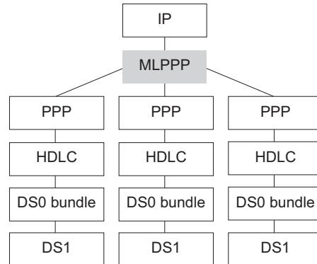
Figure 18: Interface Stacking with MLPPP
