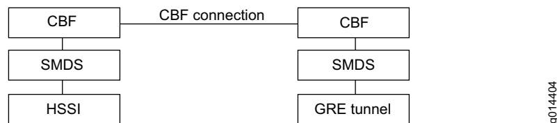
Figure 15: CBF Connection Between CBF/SMDS Interfaces
