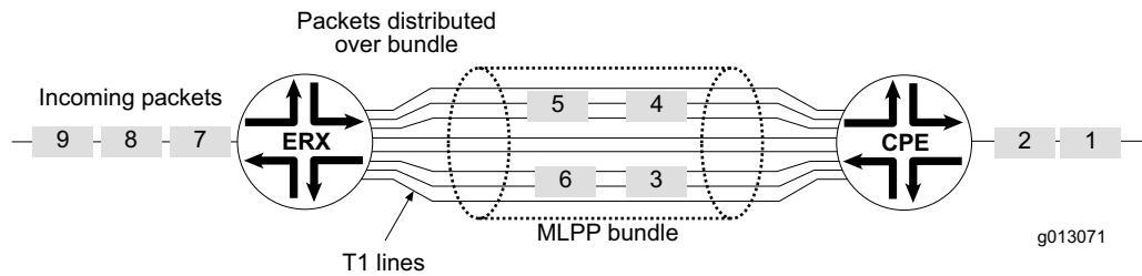
Figure 6: MLPPP aggregation of T1 lines into a single bundle
