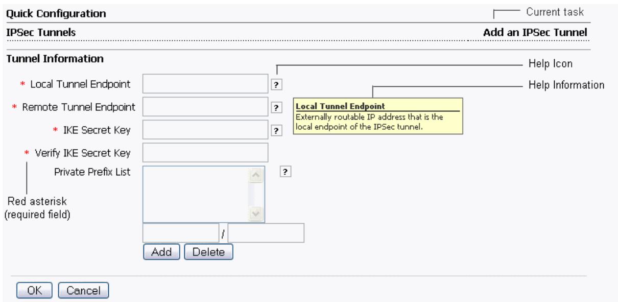
Figure 5: Main Pane Elements
