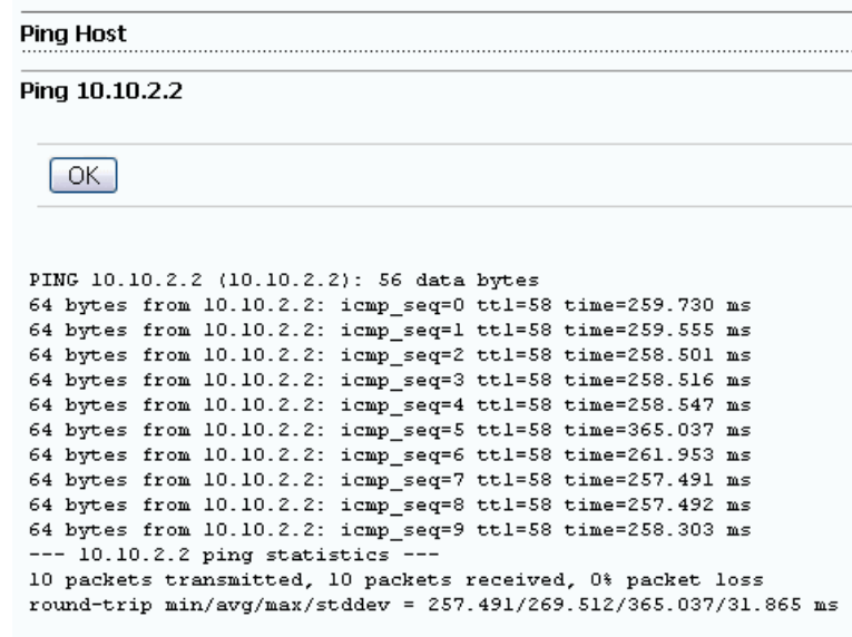
Figure 29: Successful Ping Host Results Page
