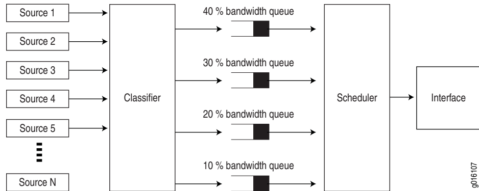
Figure 5: CoS Classifier, Queues, and Scheduler
