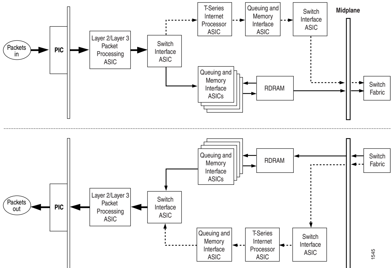
Figure 4: T-series Packet Forwarding Engine Components and Data Flow
