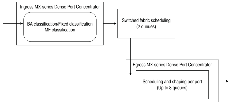
Figure 3: MX-series Packet Forwarding and Data Flow
