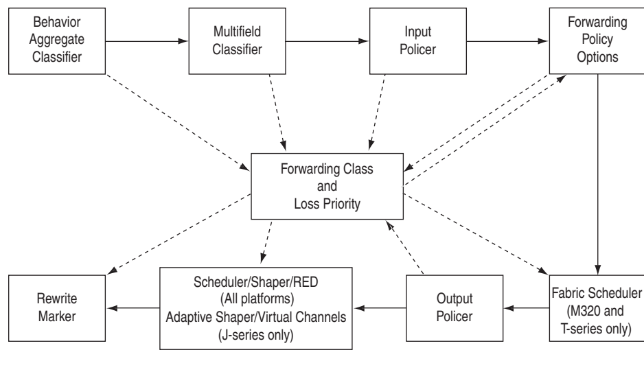
Figure 6: Packet Flow Through CoS Configurable Components
