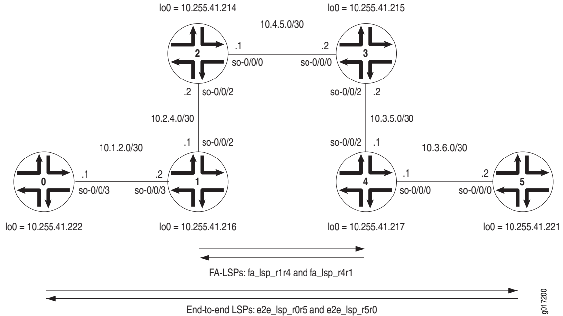
Figure 30: RSVP LSP Tunnel Topology Diagram
