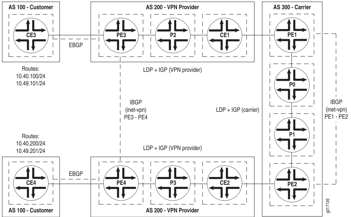
Figure 26: Multiple-Instance LDP Topology Diagram
