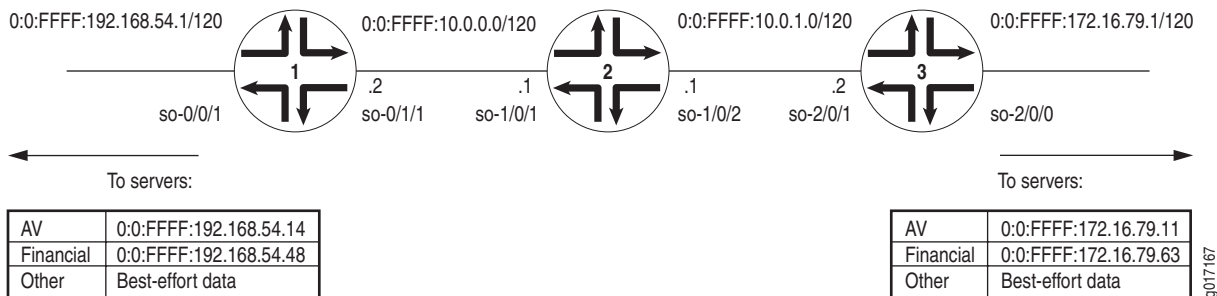
Figure 13: IPv6 DiffServ Configuration
