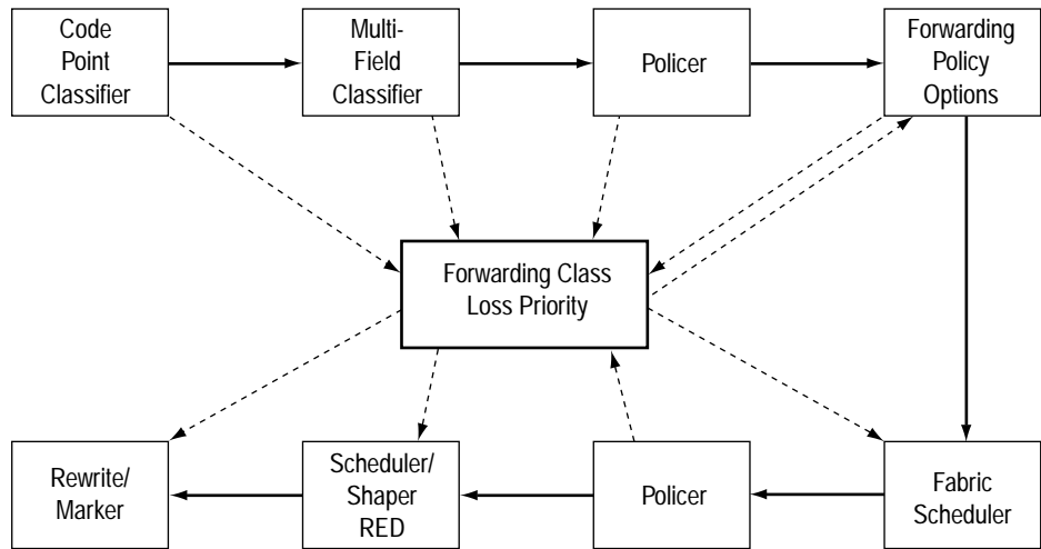
Figure 11: Packet Flow Through CoS-Configurable Components
