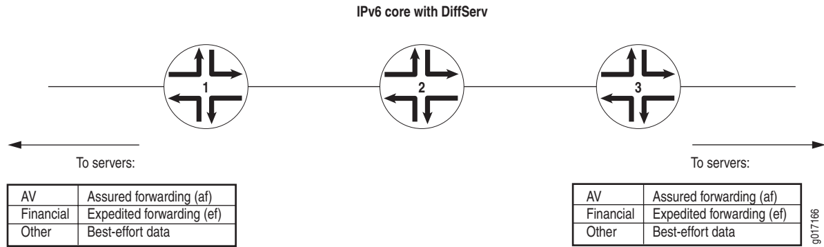
Figure 12: Basic IPv6 DiffServ Topology
