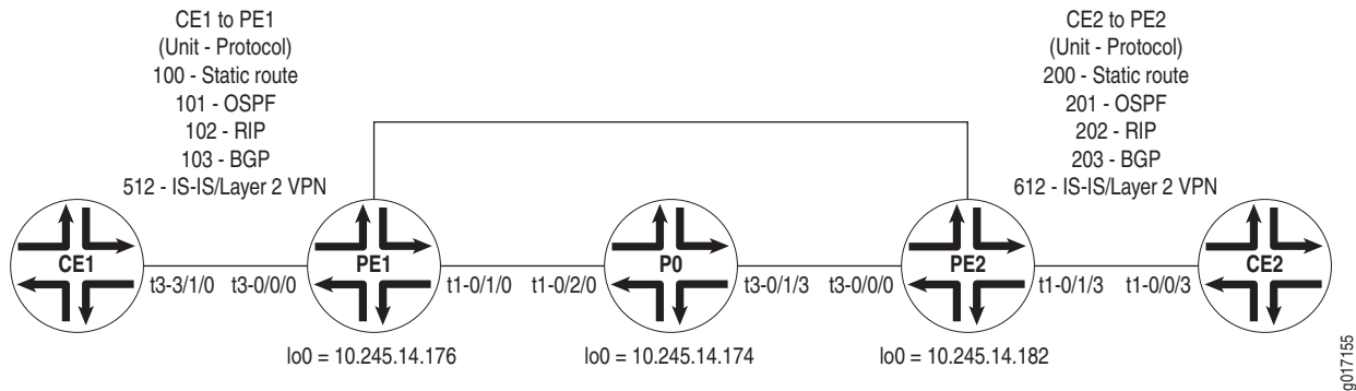
Figure 34: Layer 3 VPN Graceful Restart Topology Diagram
