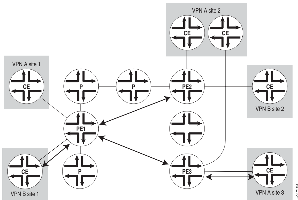
Figure 12: Route Distribution Within a VPN
