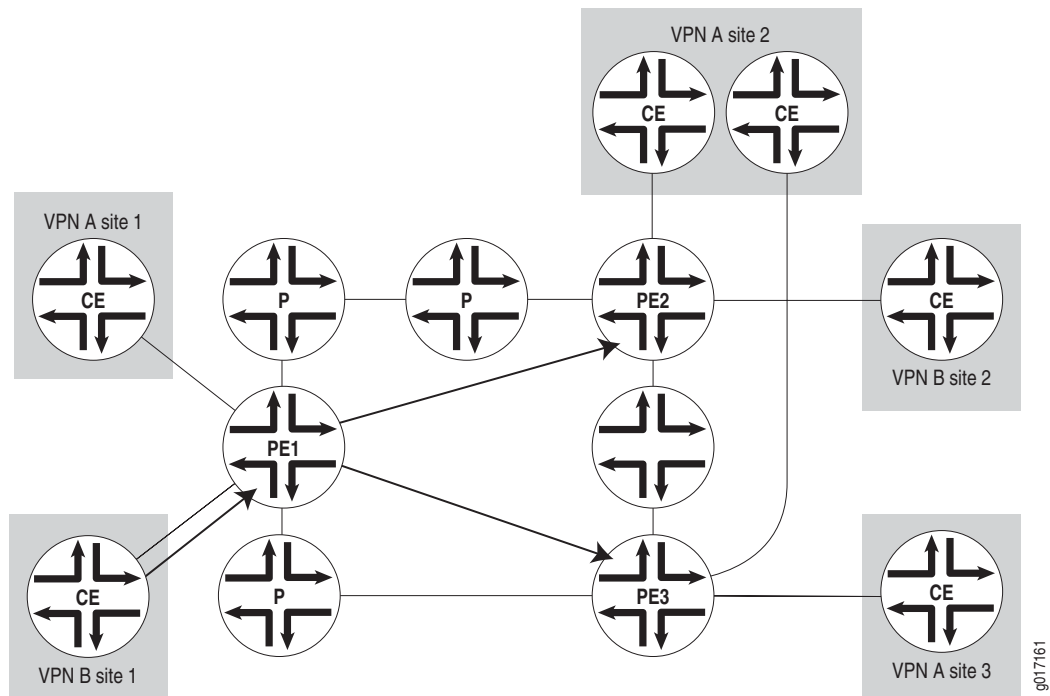
Figure 14: Distribution of Routes Between PE Routers
