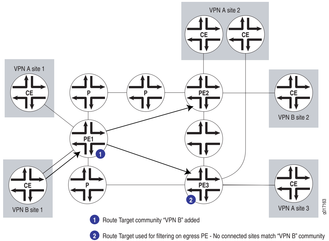
Figure 8: VPN Attributes and Route Distribution
