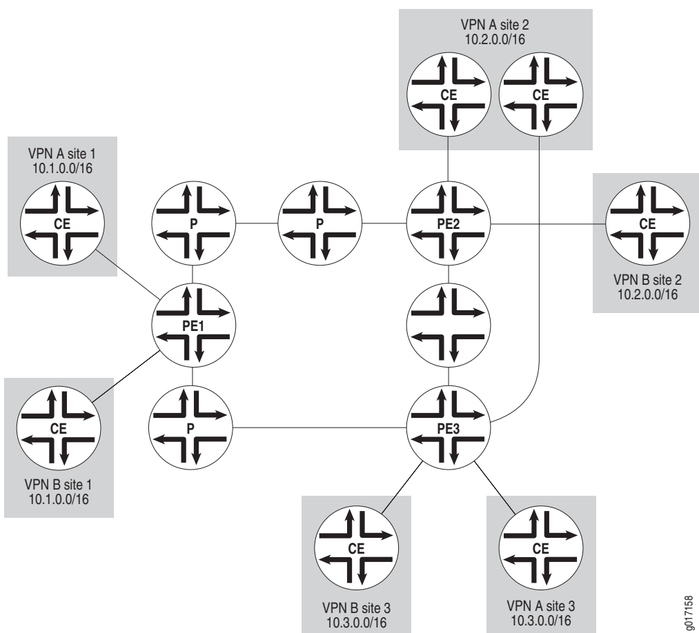
Figure 9: Overlapping Addresses Among Different VPNs
