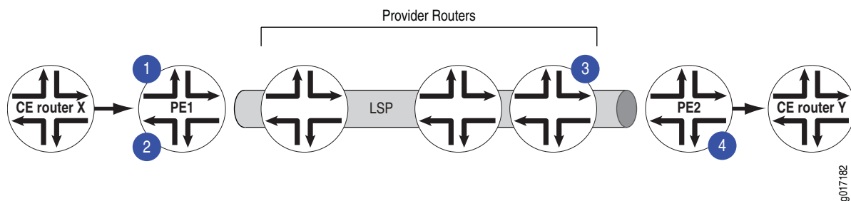
Figure 17: Label Stack
