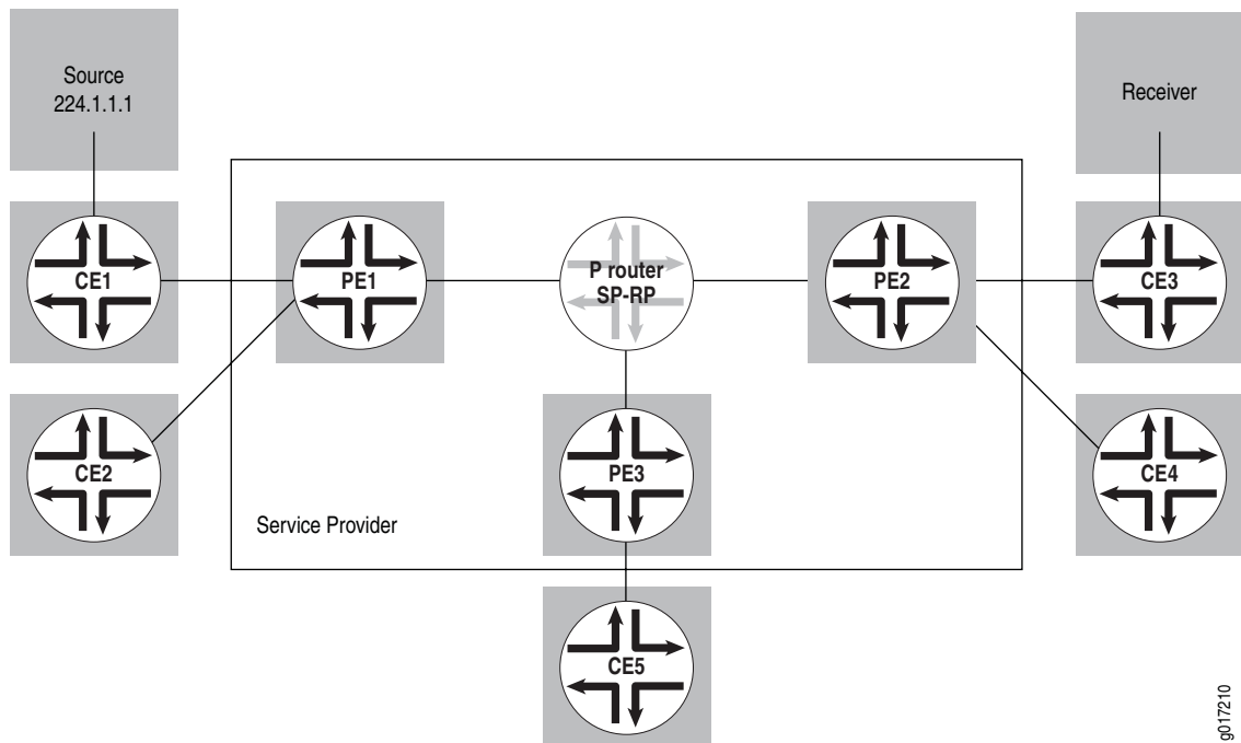
Figure 18: Multicast Topology Overview
