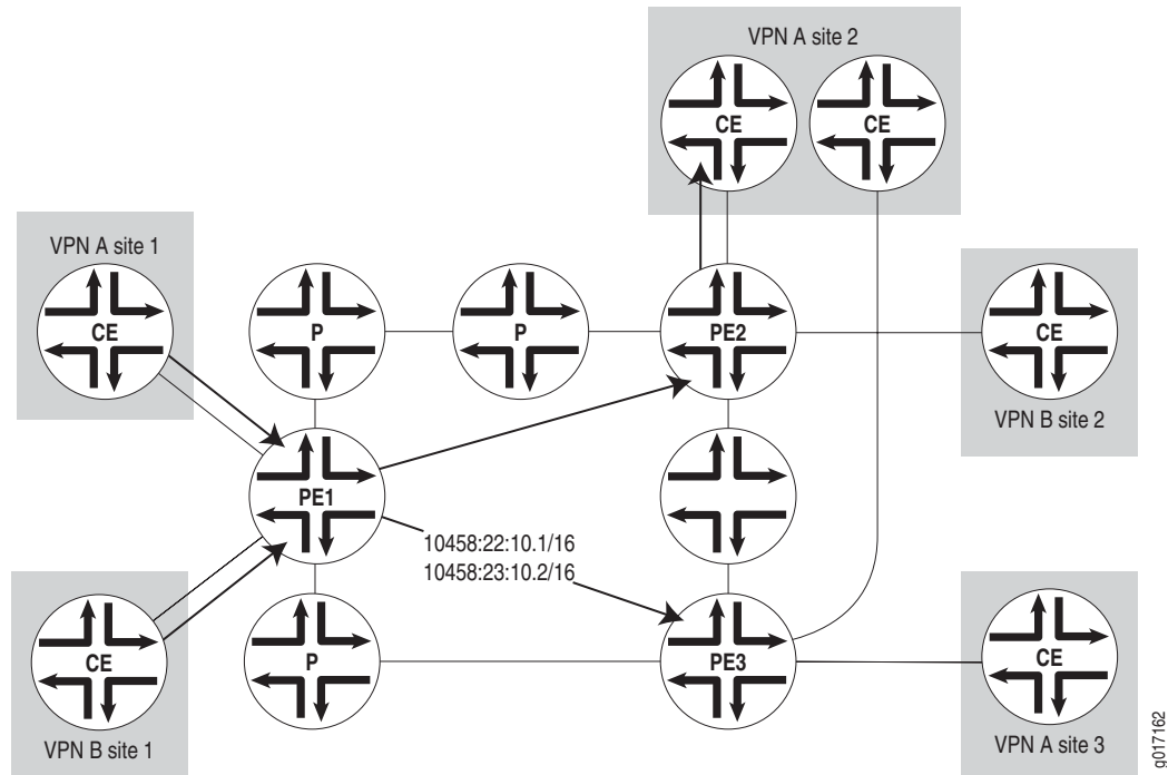
Figure 10: Route Distinguishers
