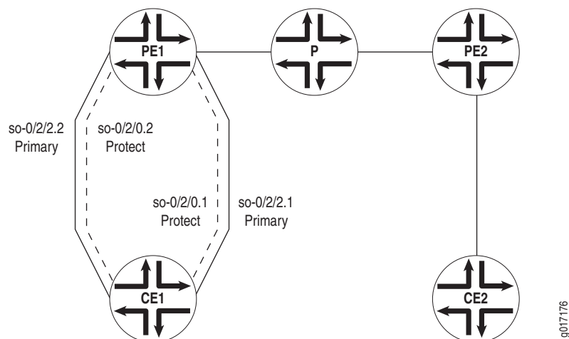
Figure 53: Layer 2 Circuits Using Protect Interfaces
