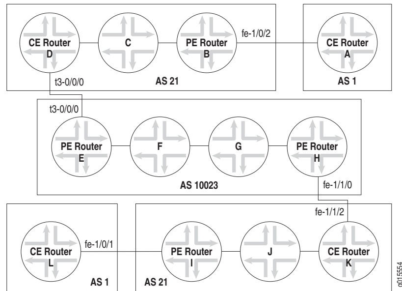
Figure 50: Carrier-of-Carriers VPN Example Network Topology
