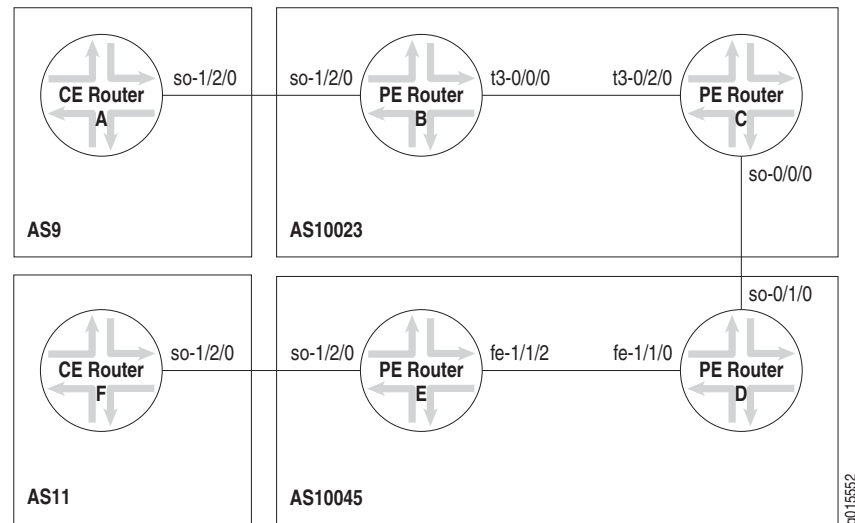
Figure 48: Network Topology of Interprovider VPN Example
