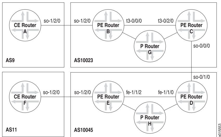
Figure 49: Network Topology of Interprovider VPN Example—Multihop MP-EBGP
