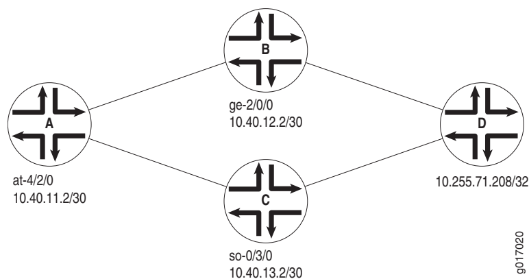
Figure 7: Sample CoS-Based Forwarding
