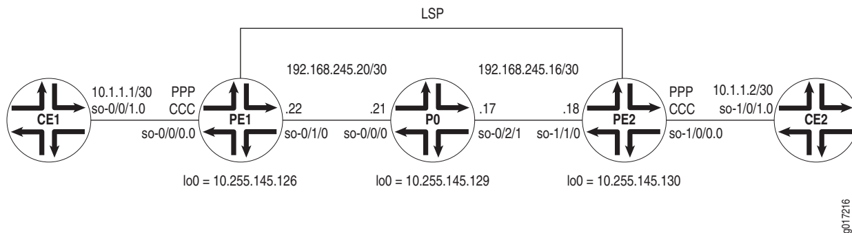
Figure 66: SONET/SDH-Based Layer 2 Circuit Topology Diagram
