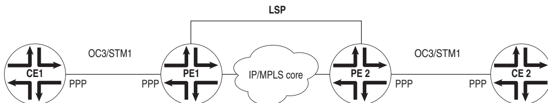
Figure 63: Layer 2 Circuit Connection
