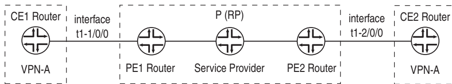
Figure 34: Customer Edge and Service Provider Networks
