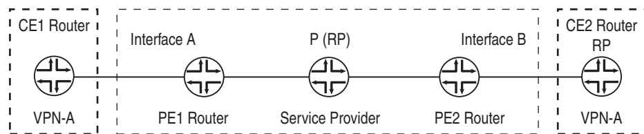
Figure 32: Multicast Connectivity on the CE Routers
