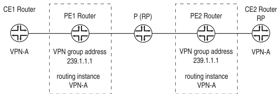
Figure 33: Multicast Connectivity for the VPN
