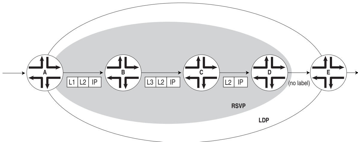
Figure 24: Double Push When LDP LSPs Are Tunneled Through RSVP LSPs
