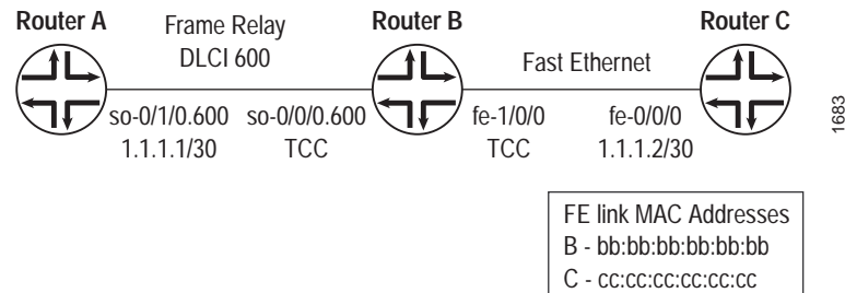
Figure 71: TCC Interface Switching—Frame Relay to Fast Ethernet
