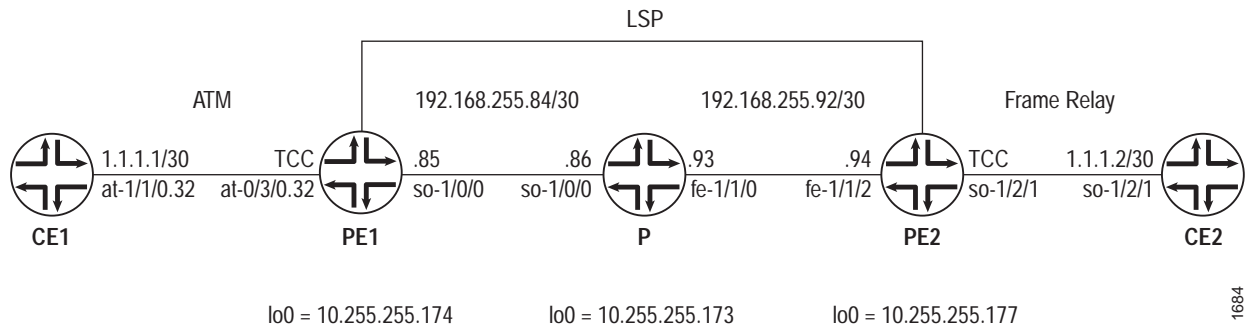
Figure 72: Layer 2.5 VPN Topology Diagram
