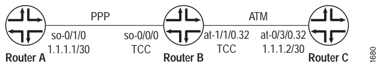
Figure 70: TCC Interface Switching—PPP to ATM
