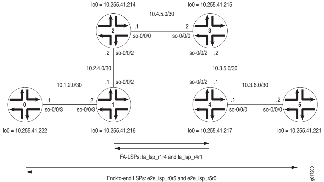
Figure 27: RSVP LSP Tunnel Topology Diagram
