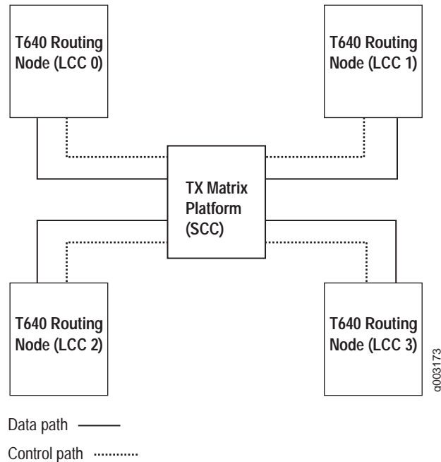
Figure 12: Routing Matrix Architecture
